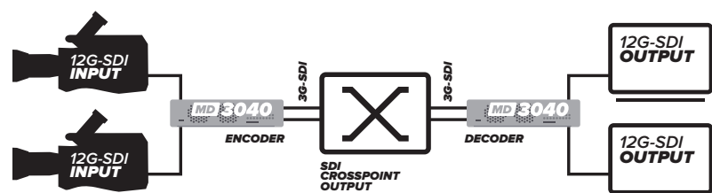
4K UHD to 3G-SDI Conversion using TICO
